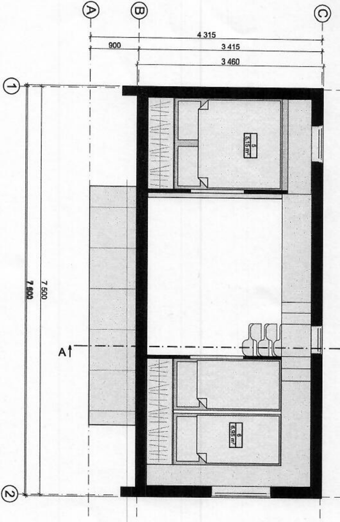
Second Floor Plan M 1:75
