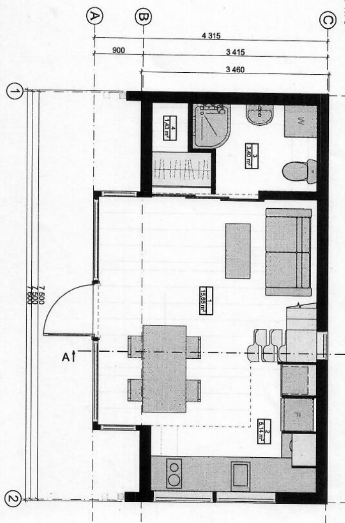
Second Floor Plan M 1:75
