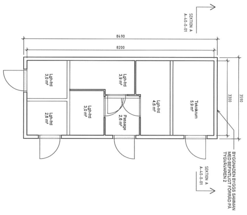
PLAN 1
