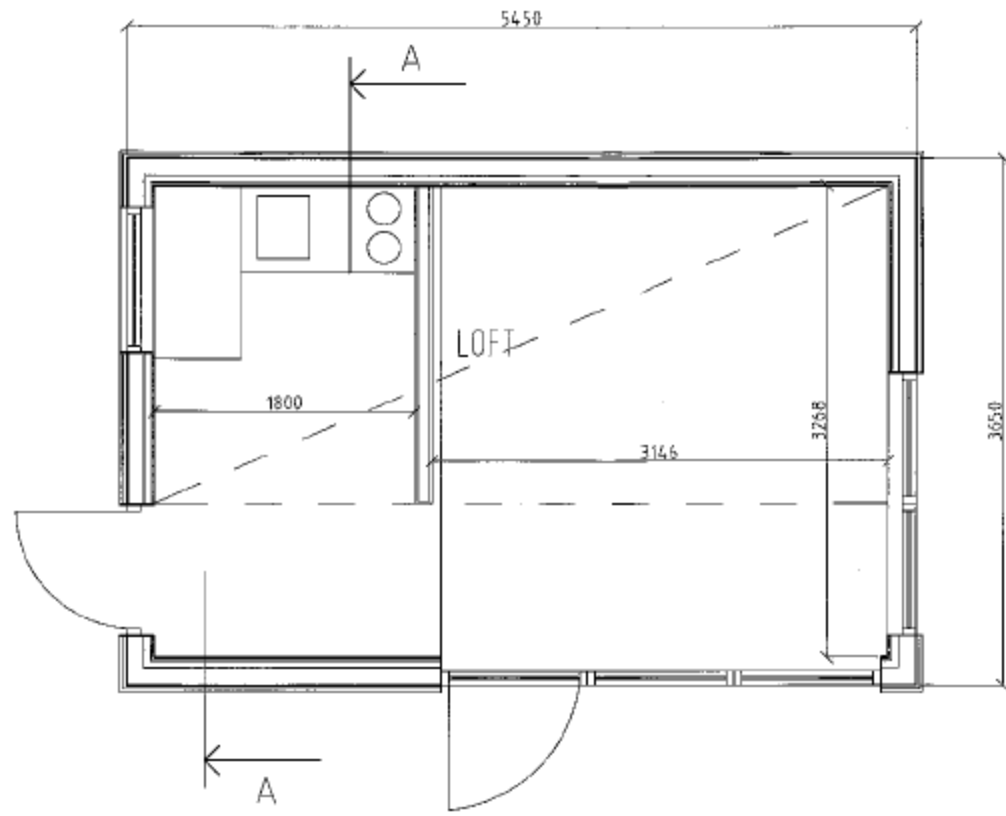
Markplan
